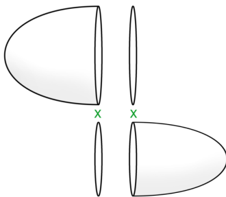
FIGURE 1. \mathbb{S}^3 \subset \mathbb{R}^5 with nonnegative curvature
