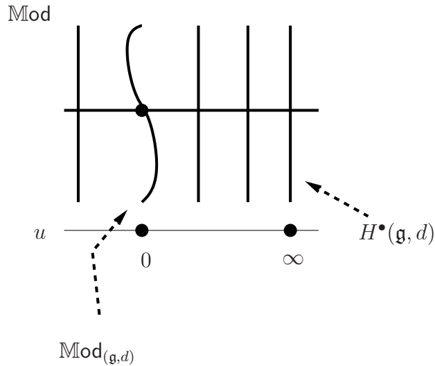
Figure 6: The relative moduli \mathbb{M}\text{od} \rightarrow \mathbb{P}^1 .
