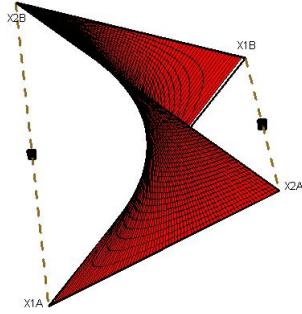
Figure 2: the surface Q = 0 in barycentric coordinates, and the two other zeros of F
