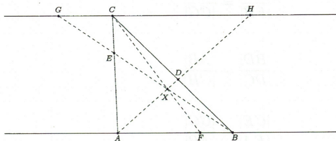
Figure 2: adding a line through C parallel to AB
