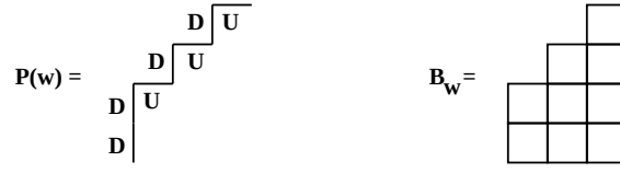
Figure 28: The rook board associated with the word w = DDUDUDU .
