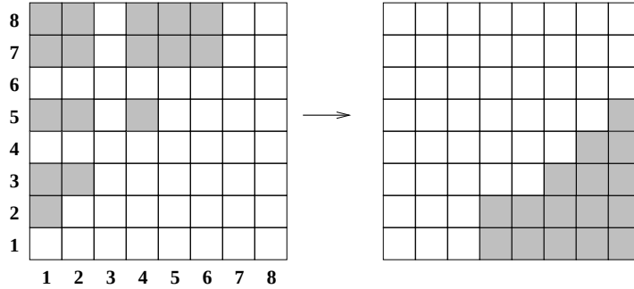
Figure 22: The board B_8^{X,Y} .
