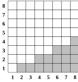
Figure 17: The Ferrers board B corresponding to B_8^{\mathbb{E}, \mathbb{N}} .
