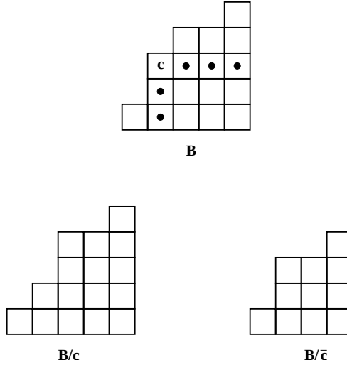
Figure 29: The boards B/c and B/\bar{c} .
