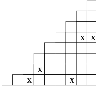
Figure 5: \Delta_9(\sigma) where \sigma = (1, 7, 3) (2, 4) (5, 9, 8) (6) .
