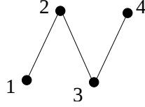
FIGURE 3. The labelled poset (P, \omega) .
