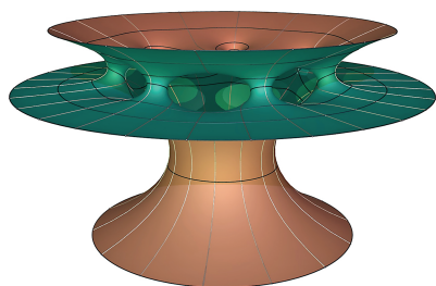
Figure 7. Hoffman–Meeks discovered how to add more handles and bend the middle end of the Costa surface.
