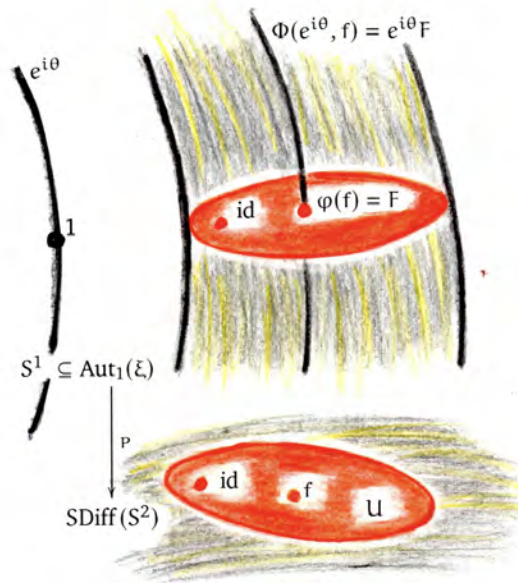
FIGURE 7. Local product structure
