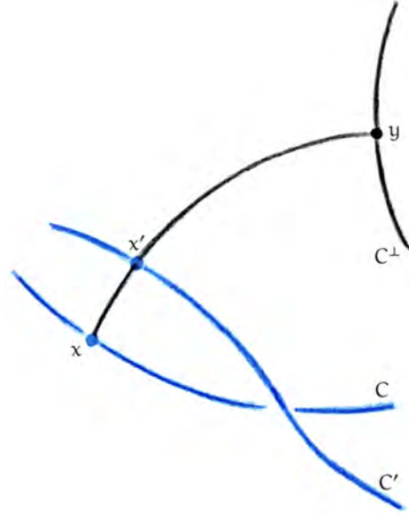
FIGURE 2. The points x and x' are nearest neighbors on the great circles C and C'
