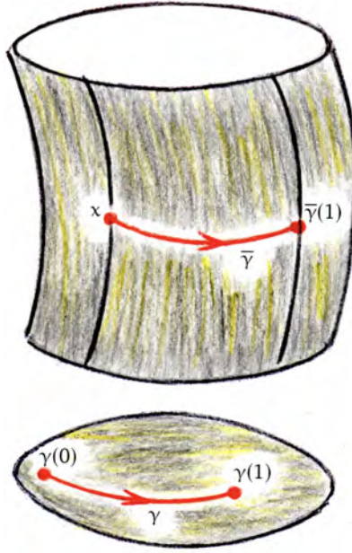
FIGURE 12. The path \gamma in S^2 lifts to the horizontal path \bar{\gamma} in S^3
