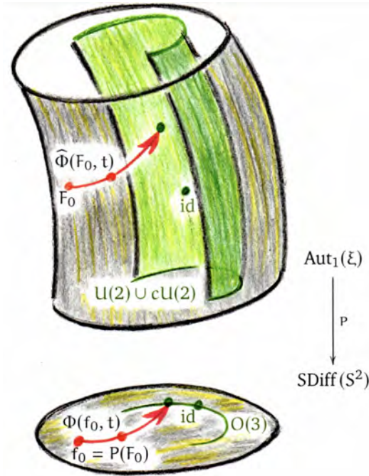
FIGURE 9. Deformation retraction of \text{Aut}_1(\xi) onto \mathcal{U}(2) \cup c\mathcal{U}(2)
