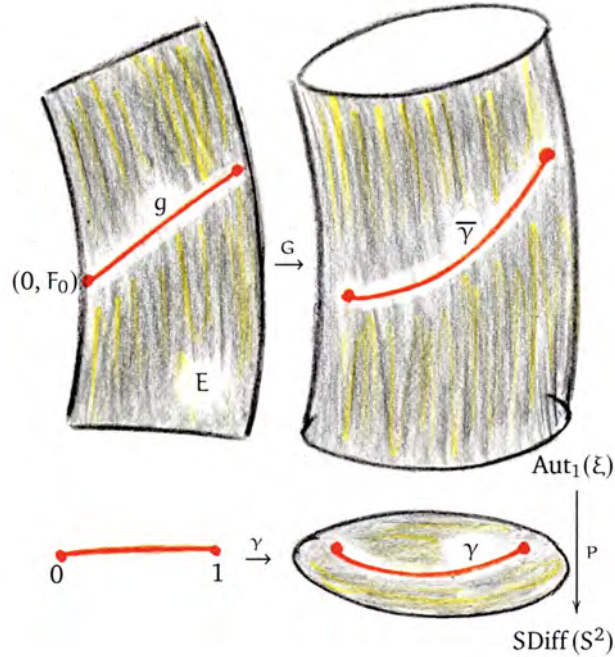
FIGURE 8. The path \gamma in \text{SDiff}(S^2) lifts to the horizontal path \bar{\gamma} in \text{Aut}_1(\xi)
