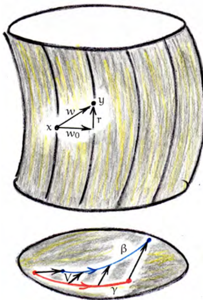
FIGURE 11. \text{Path}^* is a Fréchet manifold
