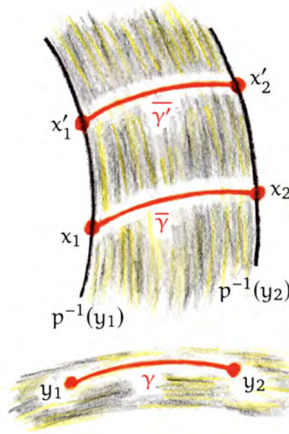
FIGURE 4. Exactness at \text{Aut}_1(\xi)
