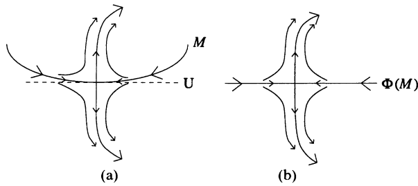
FIG. 1. (a) The flow given by \mathcal{F}(x, y) = (-x + k(x^2 - y)^4, y - 3x^2) , with stable manifold \mathcal{M} . (b) The map \Phi translates each vertical by the appropriate amount so that \mathcal{M} is mapped to U .
